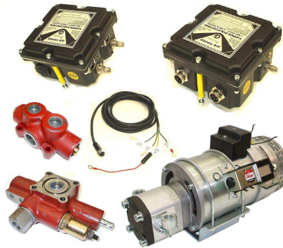
Kit "AIR-TIPPER" per FRONTALI "AIR TIPPER" kit for front mounting
